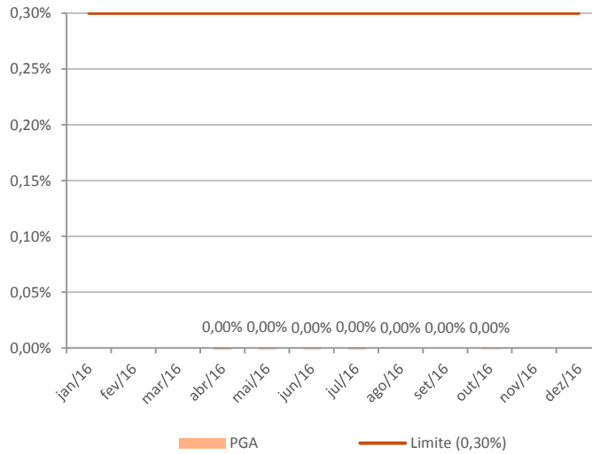
VaR - PGA
